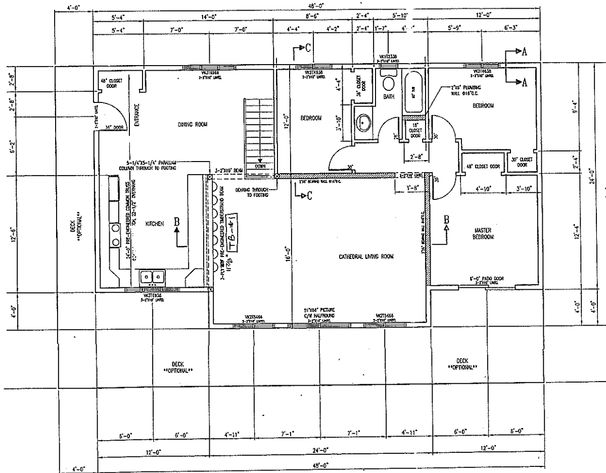
FLOOR PLAN
