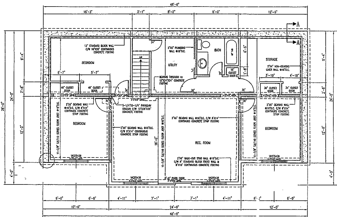
FOUNDATION PLAN
