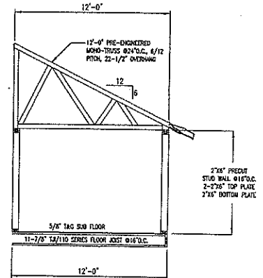
TRUSS DETAIL C-C
