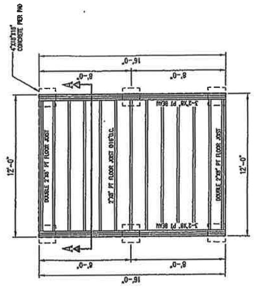
PIER PLAN
