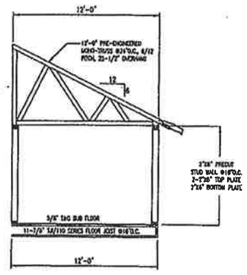
TRUSS DETAIL C-C
