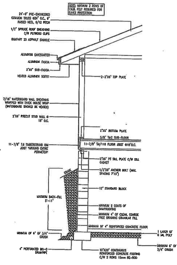
DETAIL SECTION A-A
