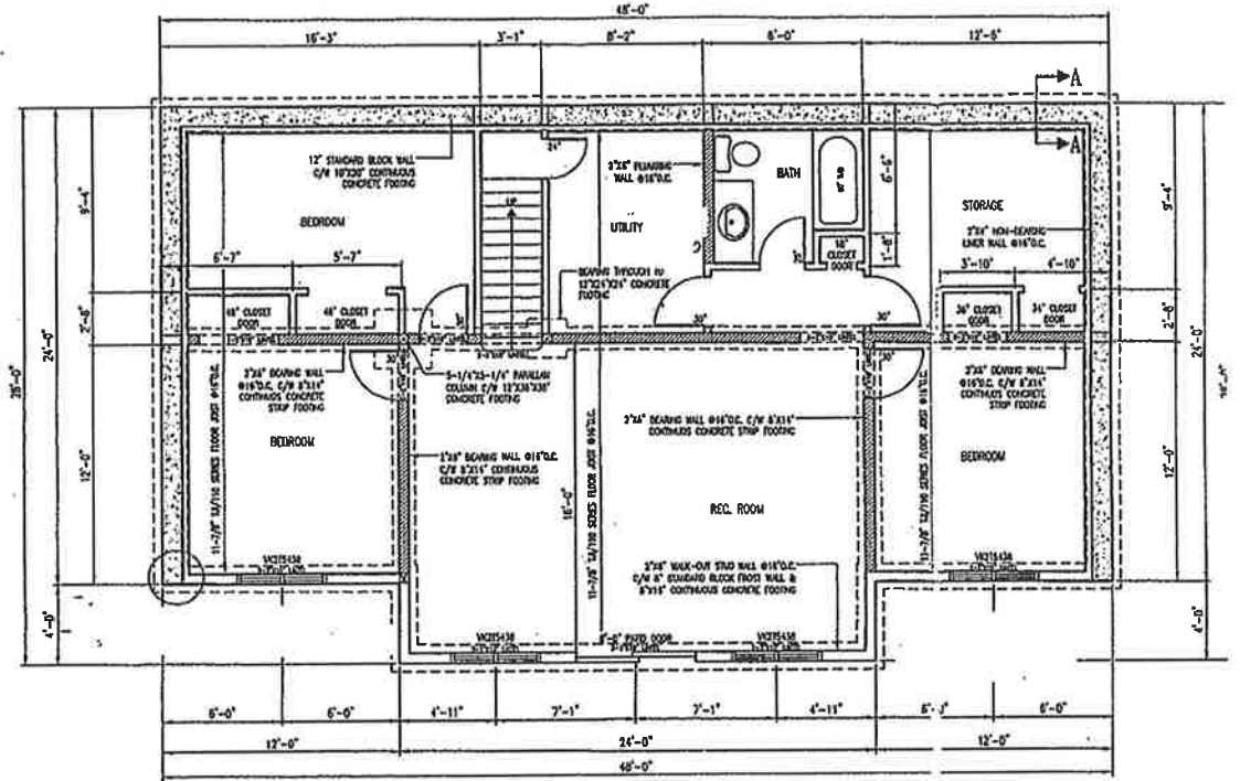
FOUNDATION PLAN
